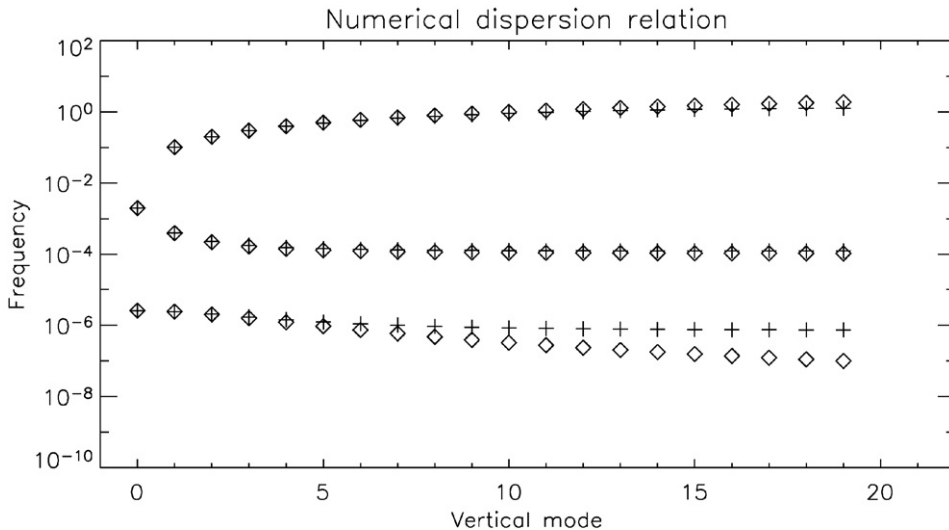
Fig. 5. Representative dispersion relation (frequency in s -1 ) for Category 2b “fast Rossby mode” configurations reproduced from [1].
