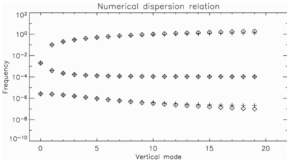
Fig. 2. Representative dispersion relation (frequency in s^{-1} ) for Category 1 “optimal” configurations reproduced from [1]. Crosses indicate numerical eigenmode frequencies and diamonds indicate analytical frequencies.
