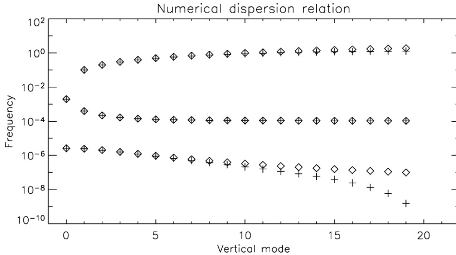
Fig. 3. Representative dispersion relation (frequency in s^{-1} ) for Category 2a “slow Rossby mode” configurations reproduced from [1].
